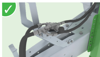
Flow regulator with compensated pressure
