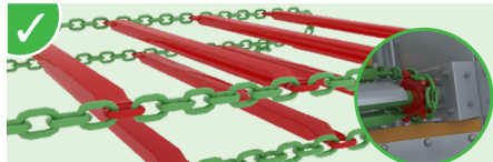
Closed tubular slats welded to Ø 14 mm shipping chains (to avoid material storage) + moulded gearwheels.
