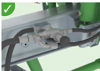
✓ Pressure regulator with compensated pressure for moving floor speed.
